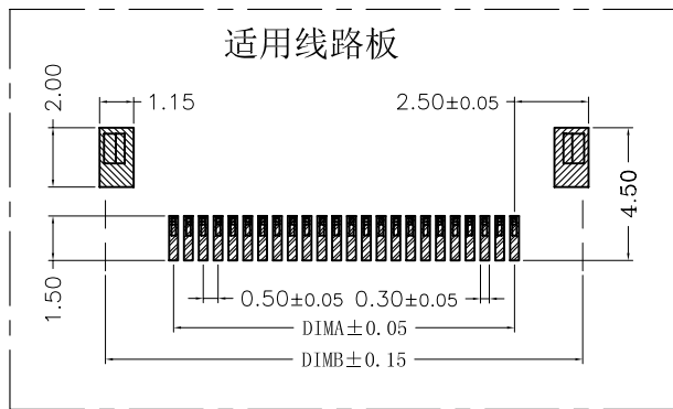
RECOMMENDED PCB Layout DEFAULT TOLERANCES: ±0.05(TOP VIEW)
