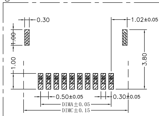
RECOMMENDED PCB Layout DEFAULT TOLERANCES:±0.05(TOP VIEW)
